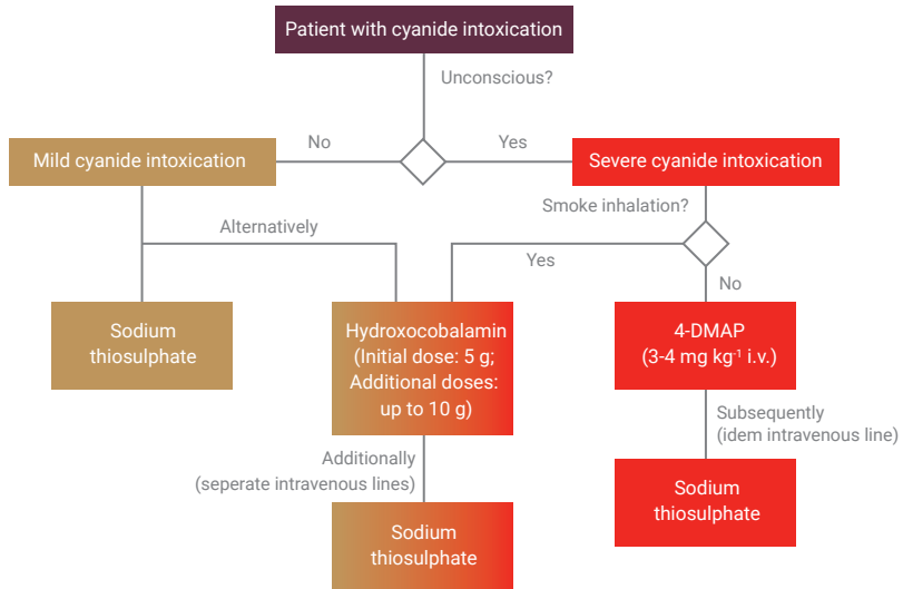
Figure 6.2 Use of the available cyanide antidotes depends on type and severity of cyanide poisoning.
