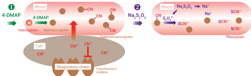
Figure 6.1 Co-administration of the methaemoglobin-forming antidote 4-DMAP and the metabolism-enhancing antidote sodium thiosulphate accelerates the cyanide clearance.
